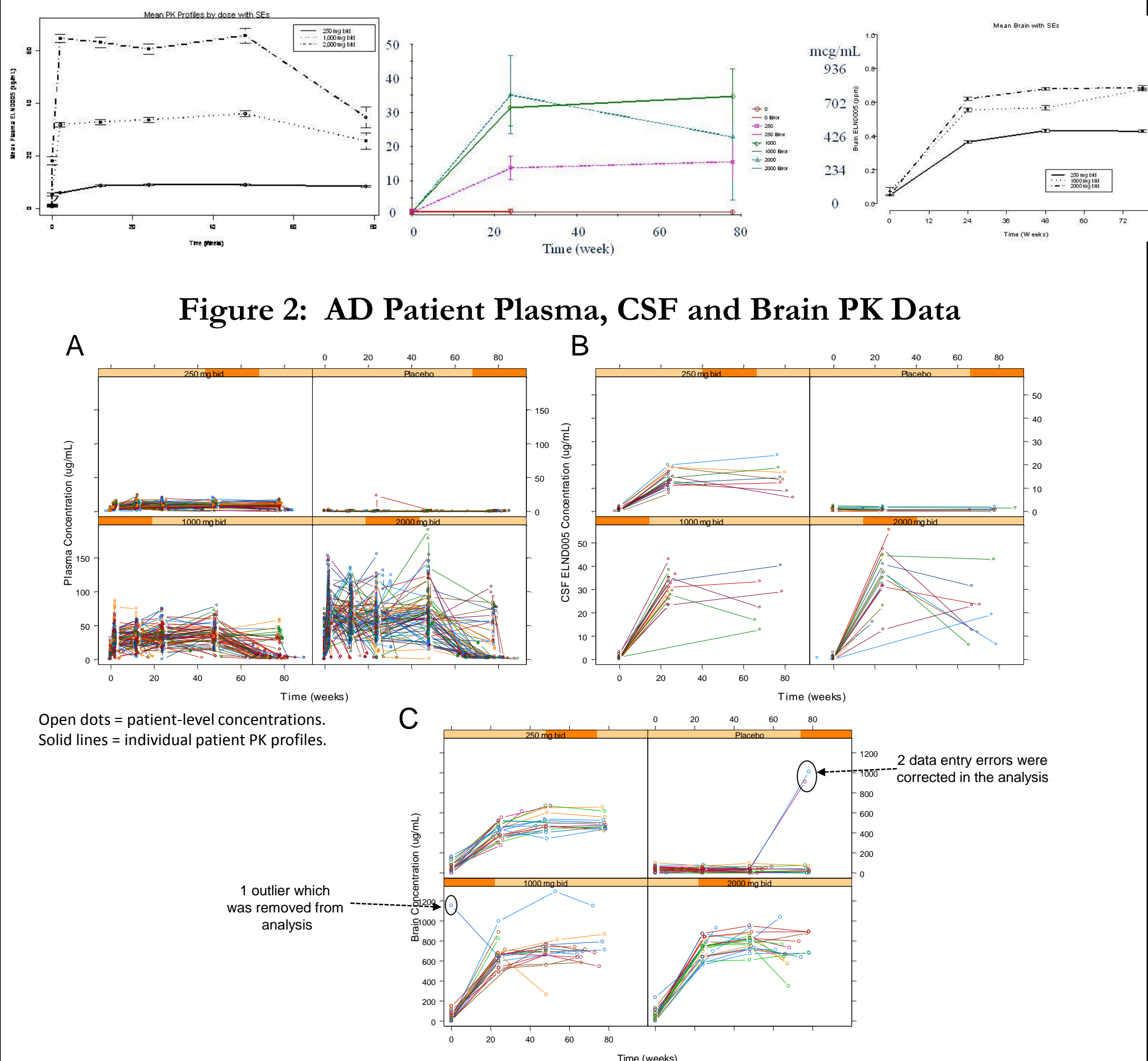
Figure 1: Concentration-Time Profiles of ELND005 in Plasma (left), CSF (middle), and Brain (right) in Study AD201
